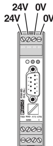
Figure 15 Connecting the supply voltage
