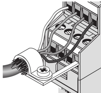
Figure 12 Install shield connection clamp
