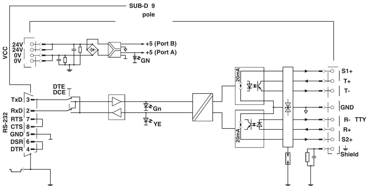
Figure 3 Block diagram
