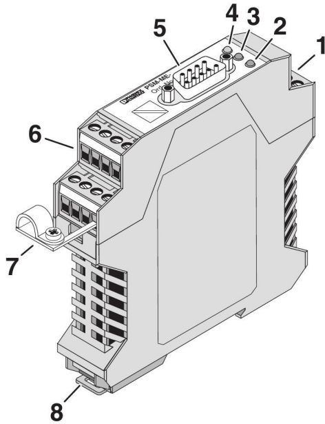
Figure 4 Function elements
