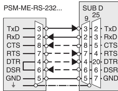
Figure 5 RS-232 interface
